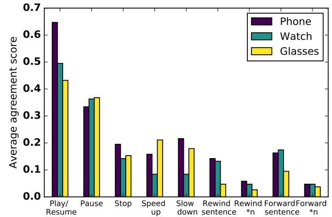
Figure 3. Agreement scores for each command on phone, watch and glasses (*n indicates several sentences).
